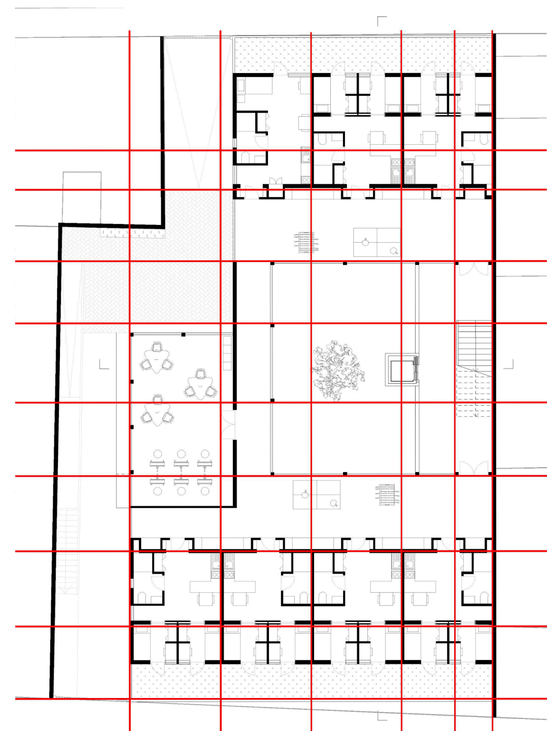
Plan R+1
