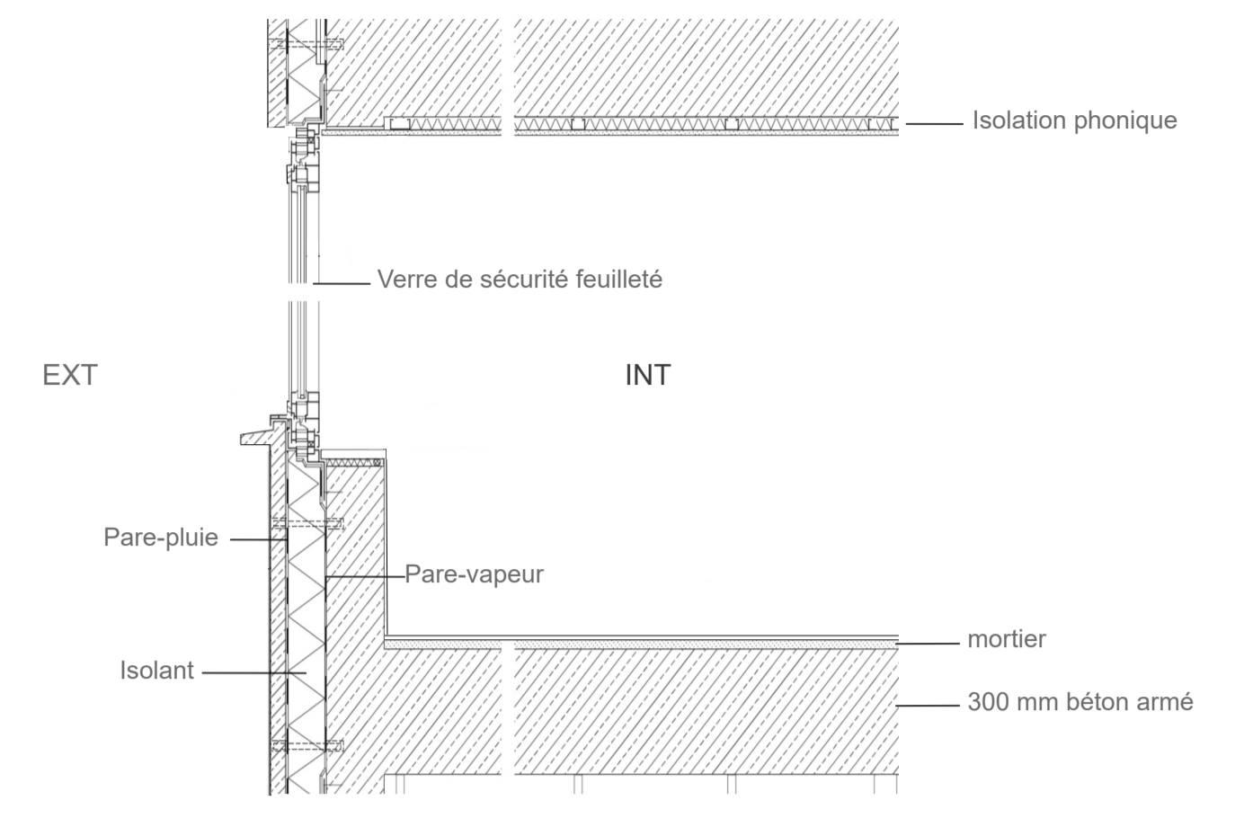
Façade
