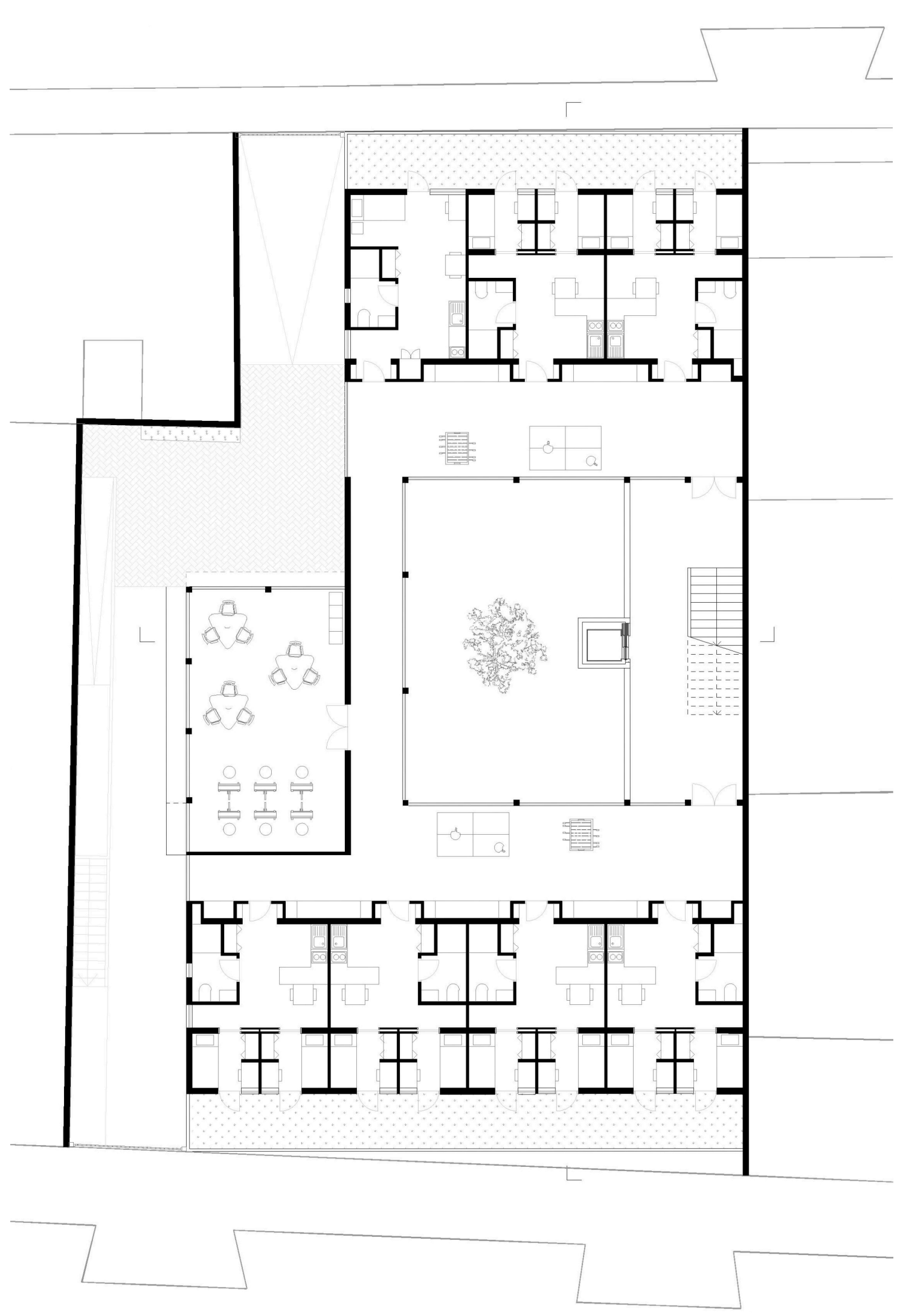
Plan R+1
