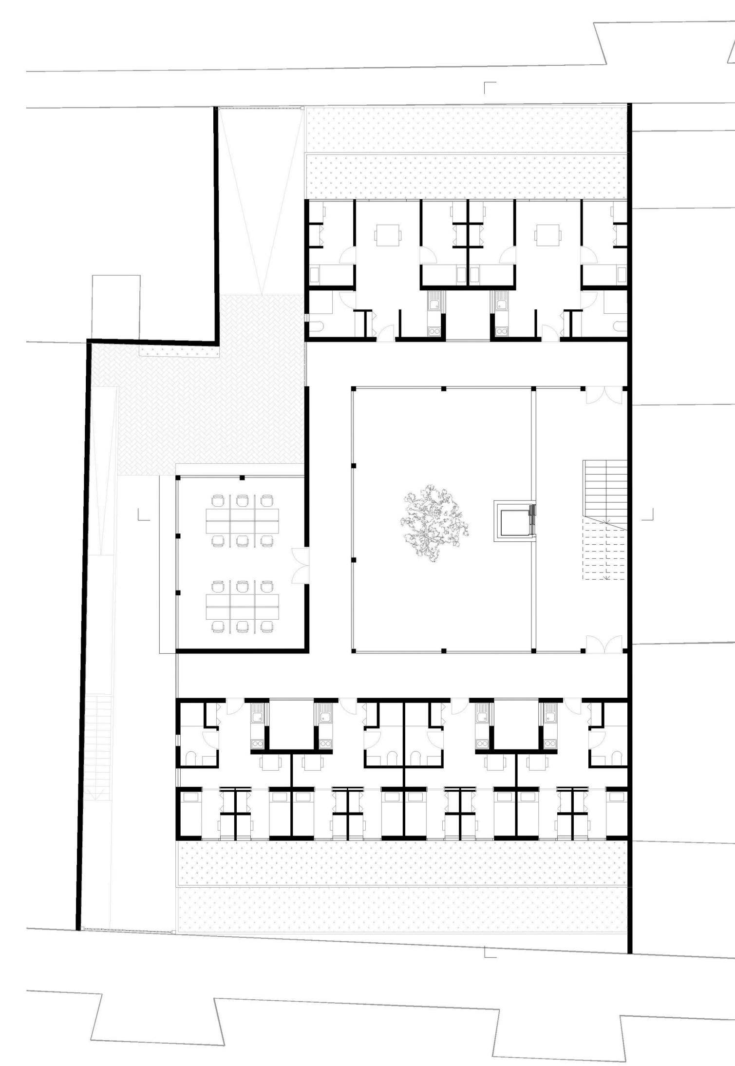
Plan R+3
